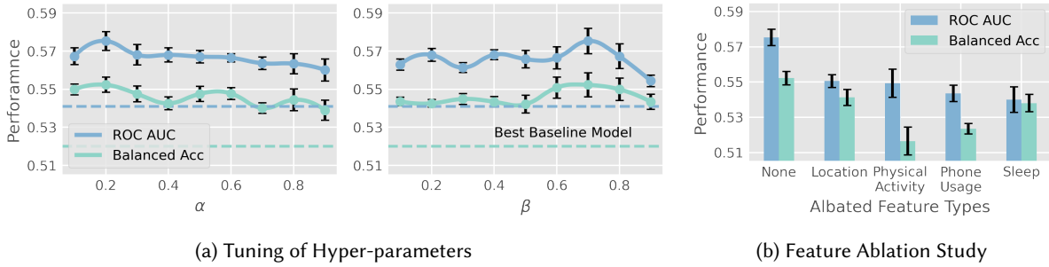
Fig. 10. Extra Experiments on Reorder to Better Understanding the Model and Features. The experiments use the leave-one-dataset-out setup to ensure consistency. The dashed line indicates the performance of the best baseline models.
